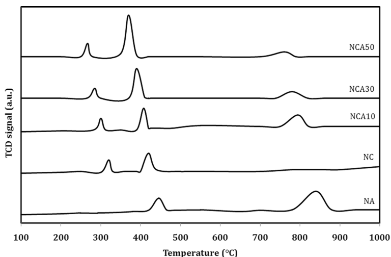
Fig.3 H 2 -TPR results for all samples
